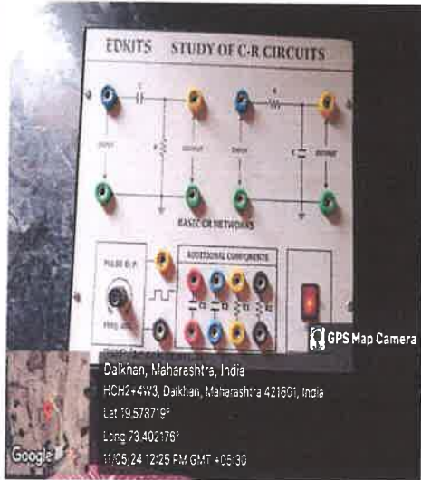
C-R Circuit
