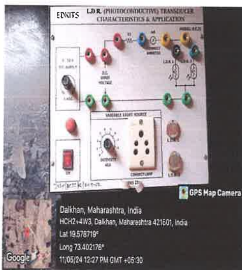
LDR Transducer Charcteristics and Application
